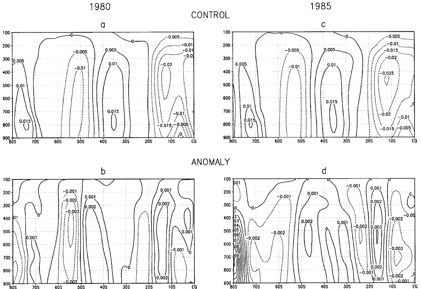
Fig. 9. Vertical cross sections ( y -axis denotes the pressure level in hPa) of the zonally averaged vertical velocities ( \text{Pa s}^{-1} ) for the (a) control and (b) anomaly (perturbations minus the controls) of 1980 and the (c) control and (d) anomaly of 1985. (Note: Results displayed in the vicinity of the Antarctic plateau are fictitious i.e. below \sim 700 hPa and poleward of \sim 75^\circ S. They have been artificially generated by interpolation to pressure levels, even though these levels are below the earth's surface)
